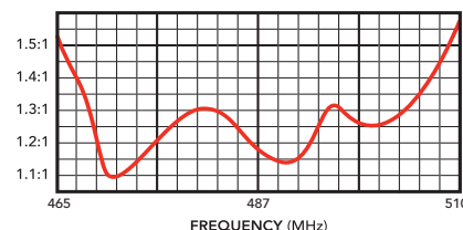
TYPICAL VSWR RESPONSE
