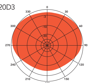
H-Plane gain 5.6 dBd Spaced 3/8 wl. from mast
