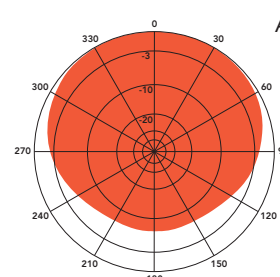
H-Plane gain 6.0 dBd Spaced 1/4 wl. from mast
