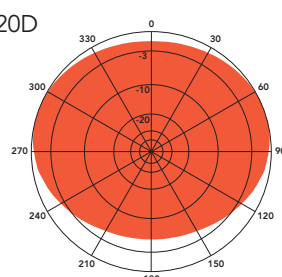
H-Plane gain 1.9 dBd Spaced 3/8 wl. from mast
