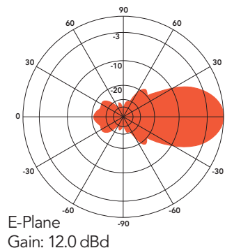
ANT2400Y12-WR at 2450 MHz
