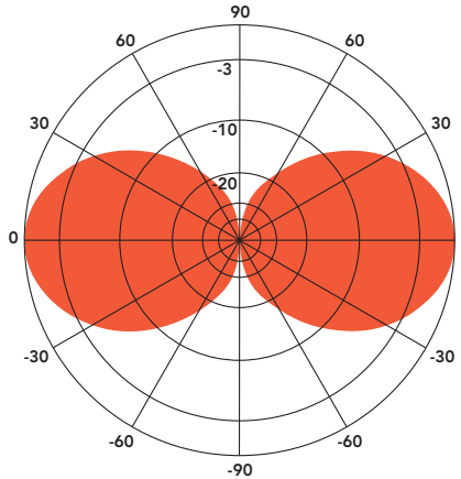
ANT960F0 - 915 MHz Vertical Plane Gain = 2.0 dBd
