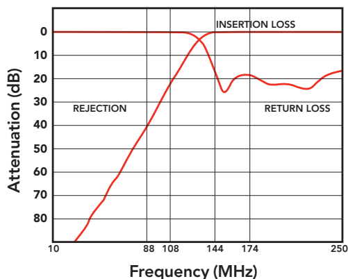
TYPICAL RESPONSE CURVE - THF-150
