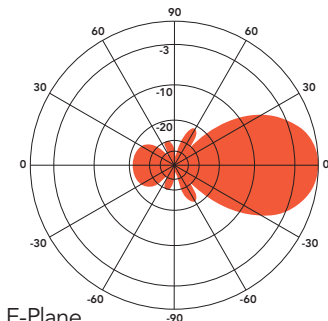
ANT450Y10-WR at 460 MHz
