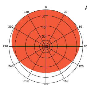
H-Plane gain 2.4 dBd Spaced 1/4 wl. from mast
